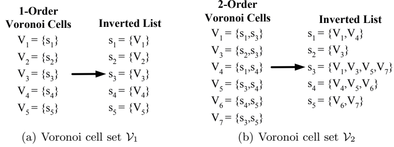
Fig. 7. Inverted lists
