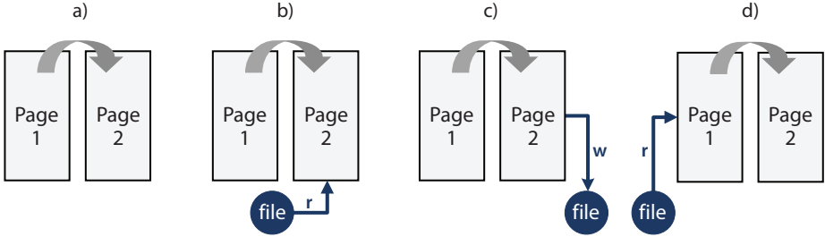
FIGURE 3. uLink can replay correctly a link to Page 2 in case a), c), and d), and in case b) if the file doesn’t change after link creation.
