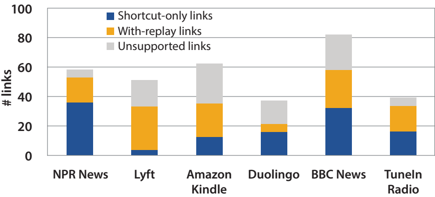
FIGURE 5. Link coverage with 6 apps (NPR News is open source, others are closed source).
