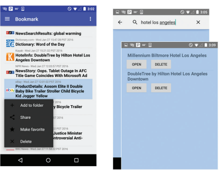
FIGURE 4. Bookmark (left) and Stuff-I’ve-Seen (right) services we have built using uLink.
